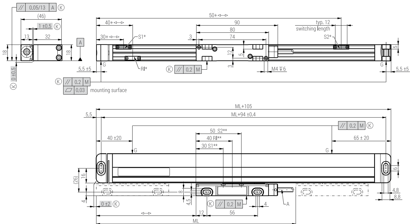
Dimensions, mounting tolerances MSA 730:
