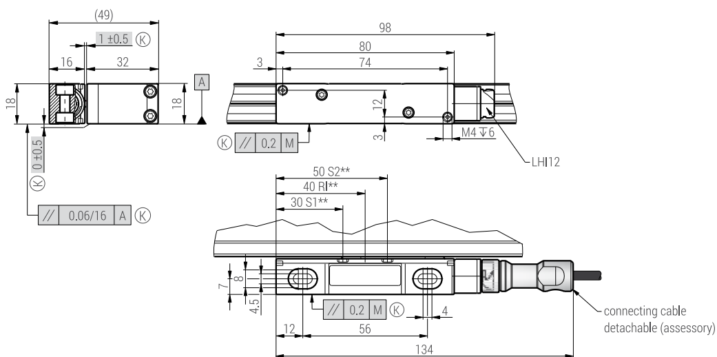
Dimensions, mounting tolerances MSA 830:
